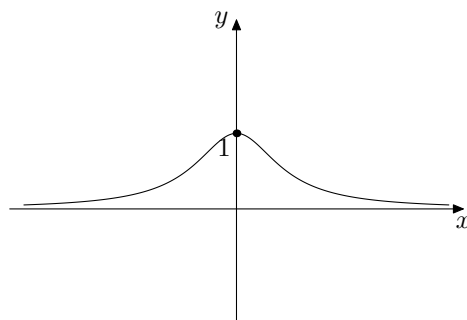
Figure 2: Graph of y = \frac{1}{2x^2 + 1}
