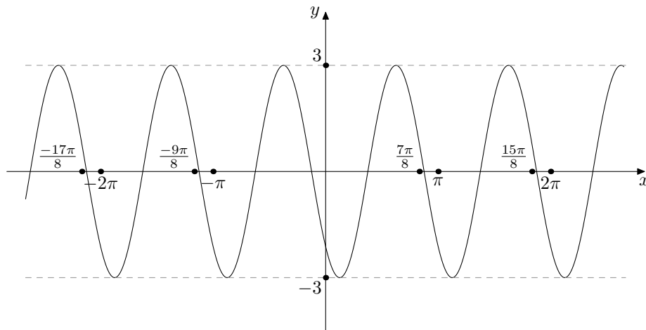
Figure 1: Graph of y = -3 \sin(2x + \frac{\pi}{4})
